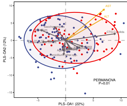
PLS-DA of Aitchison distance
