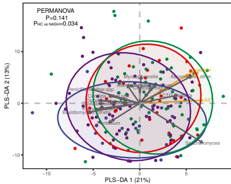
PLS-DA of Aitchison distance
