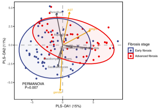
PLS-DA of Aitchison distance
